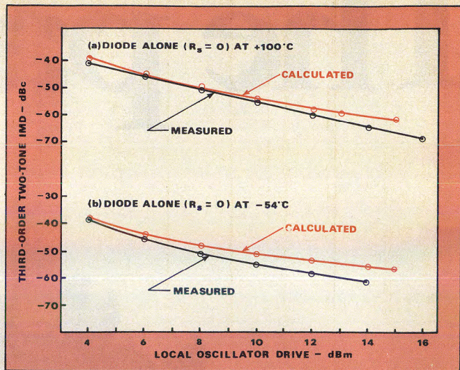
8. When internal series resistance is extracted from the computation, measured and calculated values agree closely.
