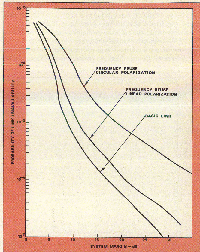
11. Availability curves prove that a linearly polarized reuse system is superior to a circularly polarized system. Neither presents as much availability as a basic link.
